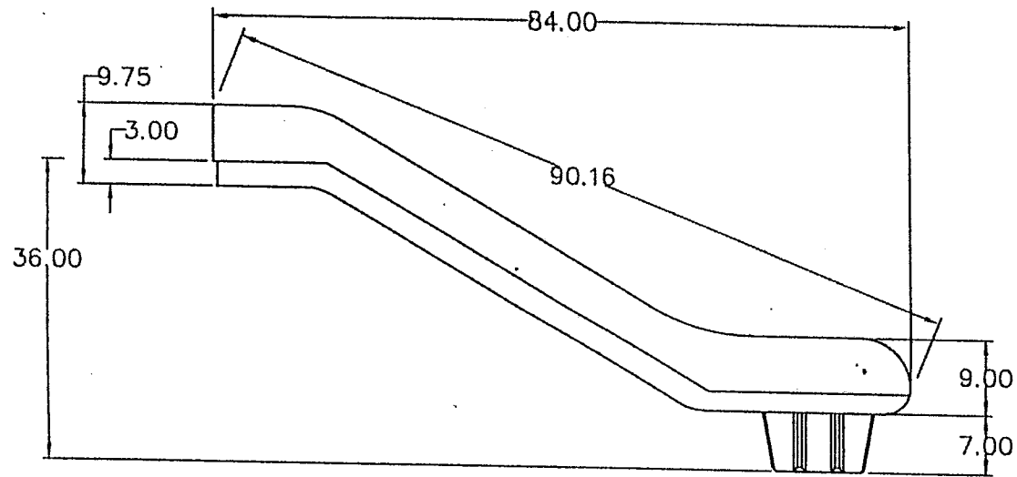
SIDE VIEW
